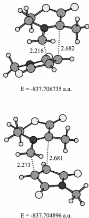
Figure 4. The endo and exo transition structures of the reaction between the model dipole and N -methylmaleimide (B3LYP/6-31G(d), distances are expressed in Å)
