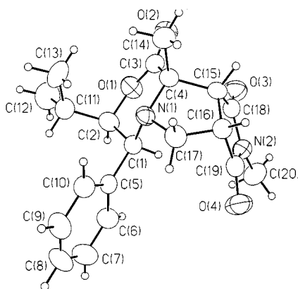
Figure 1. X-ray structure of endo adduct 14b
