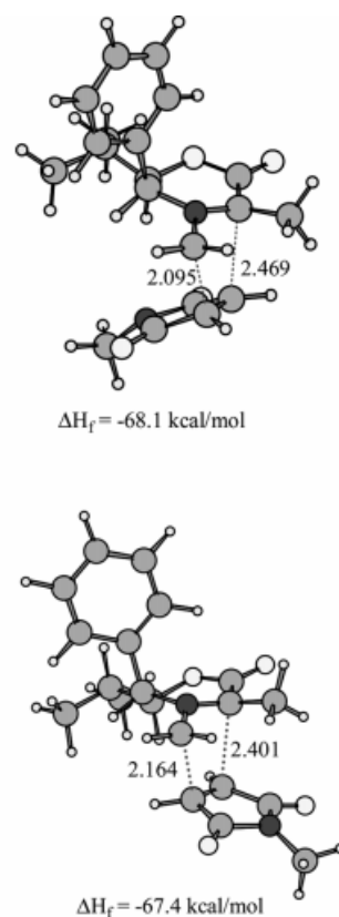
Figure 3. The endo and exo transition structures of the reaction between dipole 13 and N -methylmaleimide (PM3 Hamiltonian, distances are expressed in Å)
