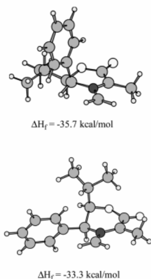
Figure 2. The two possible low energy conformations (PM3 Hamiltonian) of the dipole 13
